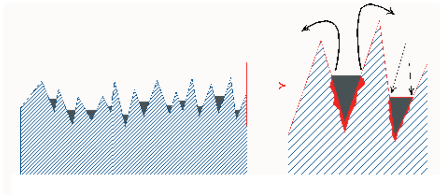
Fig. 9. Ground surface that has been significantly enlarged in the diagram. Dirt and other deposits ensure that chlorine ions, for example, are able to penetrate deeply underneath these depositions leading to local corrosion of the surface. Corrosion products such as rust will then appear.
